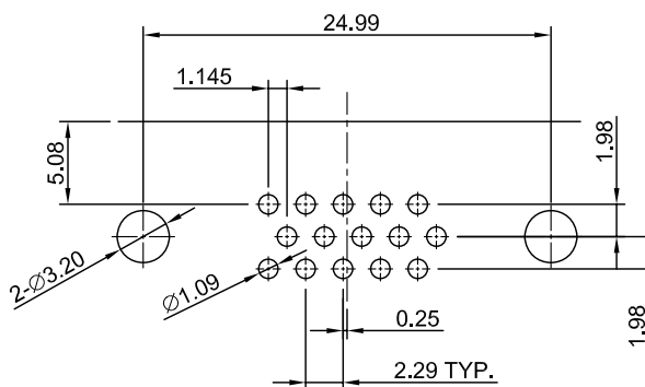
RECOMMENDED PCB LAYOUT ±0.10mm
