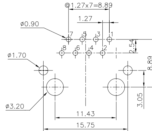
PC Board Layout t=1.6mm Component Side Show
