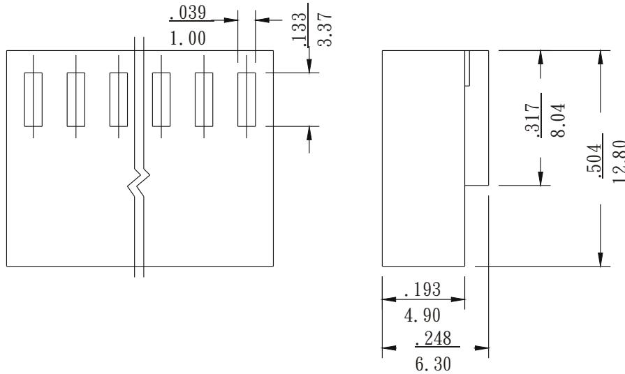
Dimensional information-inch/mm
