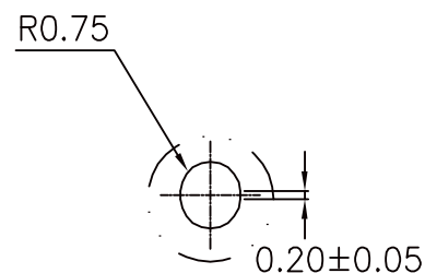
DETAIL: "A"(S=5/1)
