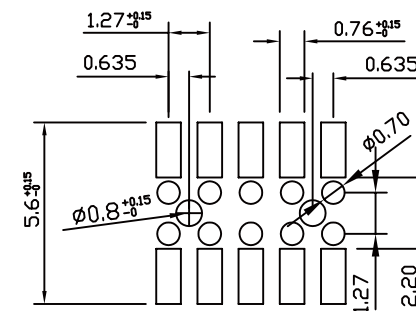
Recommended P.C. Board SMD Layout
