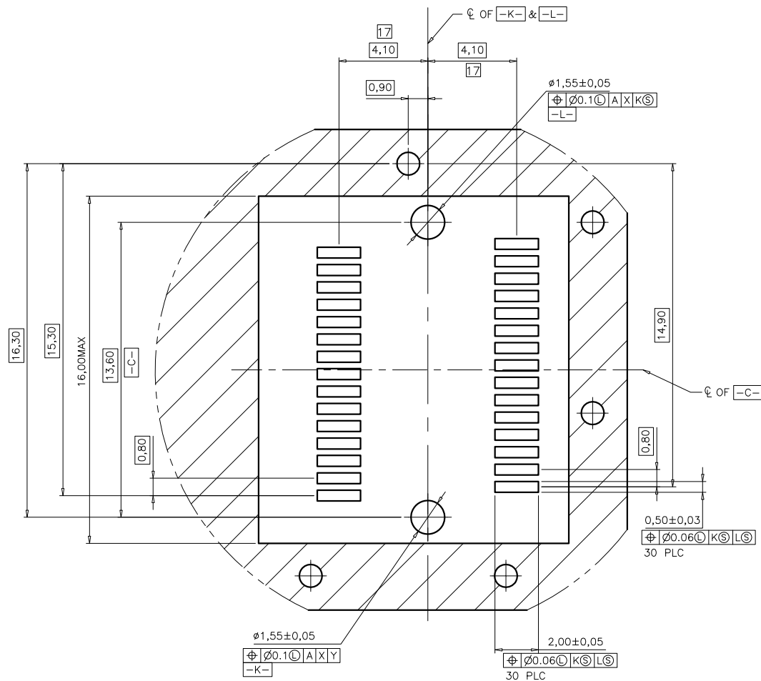
RECOMMENDED PCB LAYOUT CONNECTOR MOUNTING SIDE SCALE 2:1
