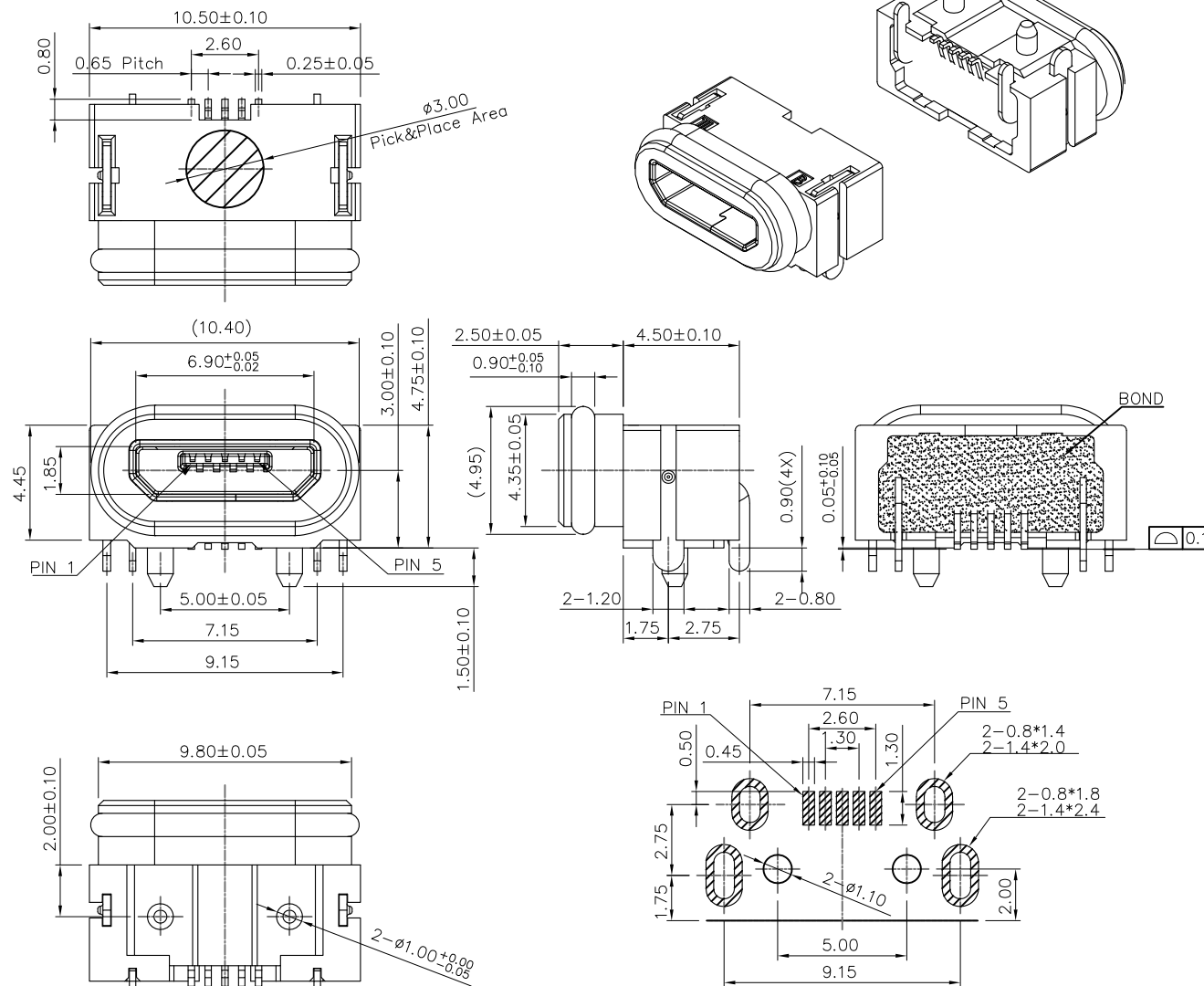
RECOMMEND PCB LAYOUT TOLERANCE: \pm 0.05 TOP VIEW
