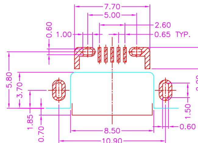
P.C.B. LAYOUT TOP VIEW \pm 0.05
