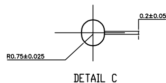
DETAIL C
