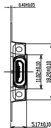
SECATION B-B
