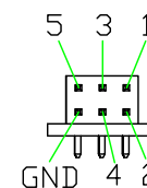
Pin Assignment Rear View (後視圖)
