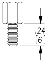
4-40 HEX JACK SCREW FOR PANEL THICKNES S BETWEEN 0.05" AND 0.078"
