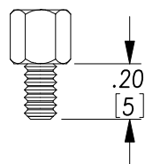
4-40 HEX JACK SCREW FOR PANEL THICKNES S UNDER 0.05"
