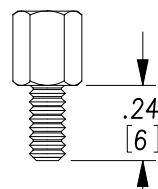
4-40 HEX JACK SCREW FOR PANEL THICKNES S BETWEEN 0.05" AND 0.078"
