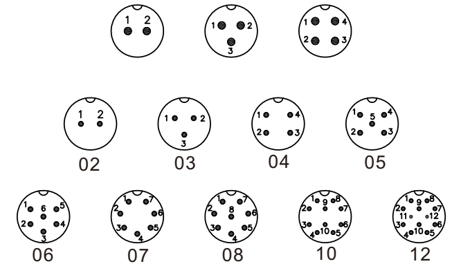
PIN ASSIGNMENT FRONT VIEW (前視圖)
