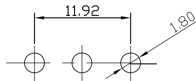
PCB LAYOUT COMPONENT SIDE
