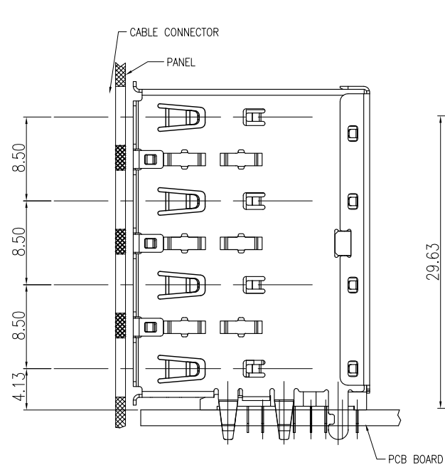
RECESSED MOUNTING CONFIGURATION
