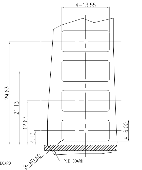
MOUNTING PANEL CUTOUT (INTERNAL SIDE)
