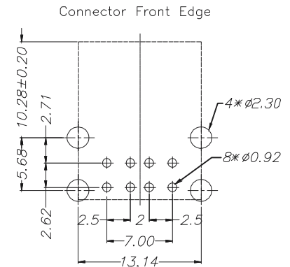
Printed Circuit Board (PCB) Layout (T=1.60mm TOL:±0.05mm)
