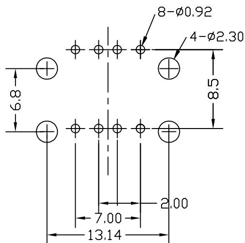
PCB LAYOUT
