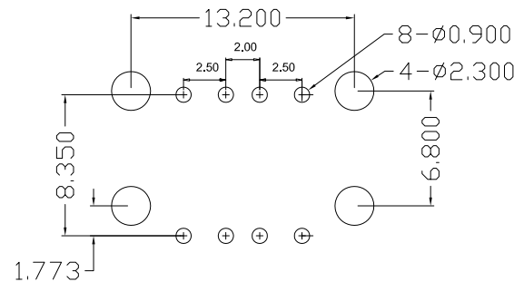
RBCOMMENDBD P.C.B PATTBRN LAYOUT
