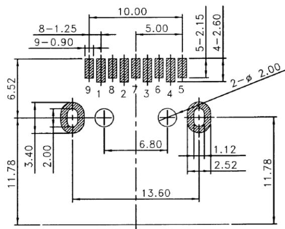
RECOMMENDED P.C.B LAYOUT TOLERANCES: ±0.05mm
