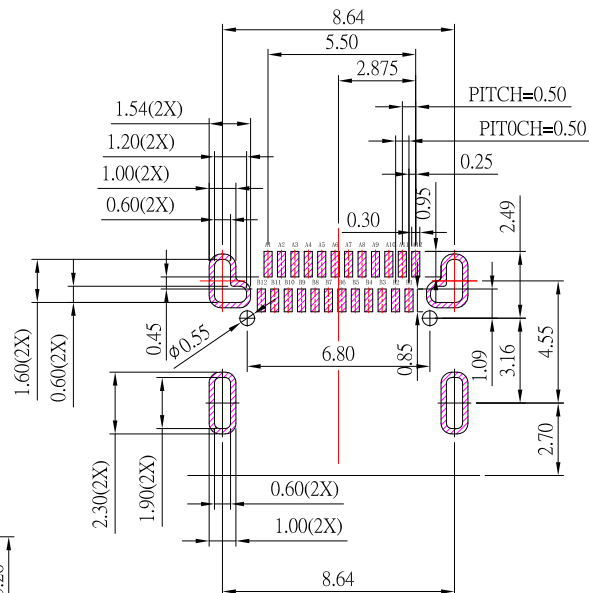
P.C.B LAYOUT MOUNTING PATTERN
