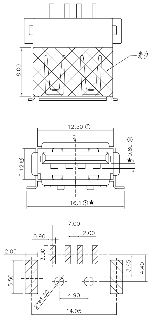
PCB.LAYOUT
