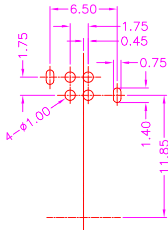
P.C.B. LAYOUT TOP VIEW \pm 0.05
