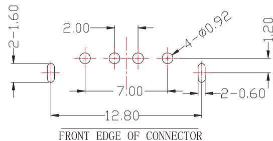
FRONT EDGE OF CONNECTOR
