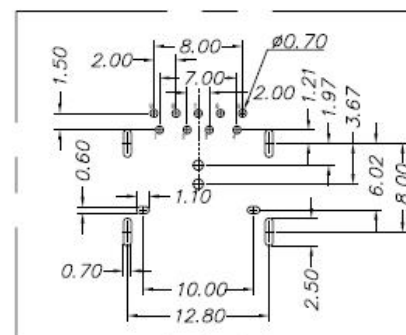
REFERENCE PCB LAYOUT TOLERANCE: \pm 0.05
