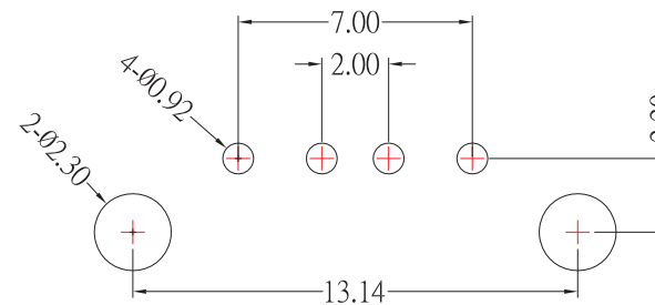
P.C.B LAYOUT MOUNTING PATTERN
