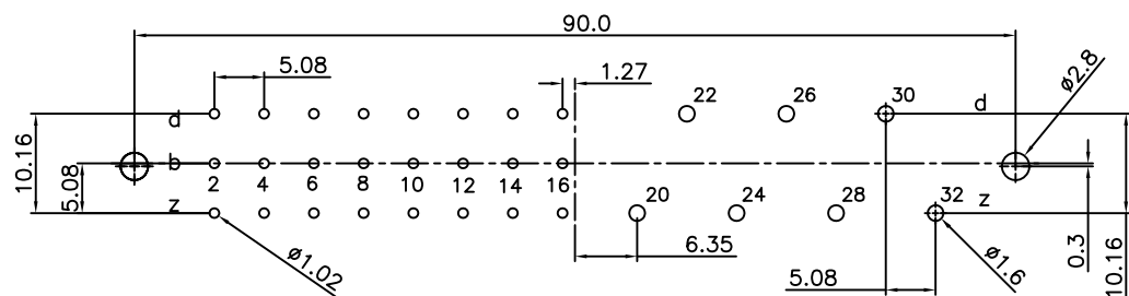
P.C. Board Layout (Tolerance: \pm 0.05 )
