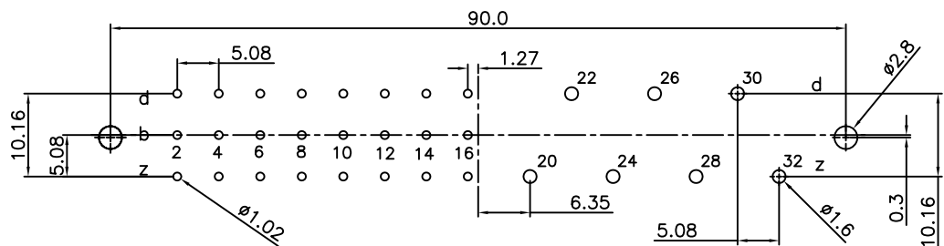
P.C. Board Layout (Tolerance: \pm 0.05 )
