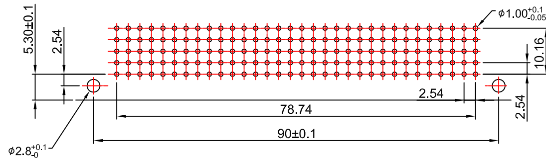
PCB LAYOUT
