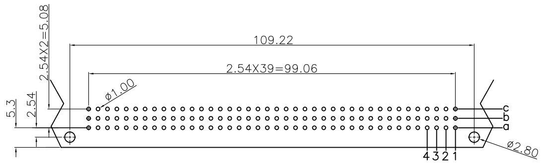
P.C. Board Layout
