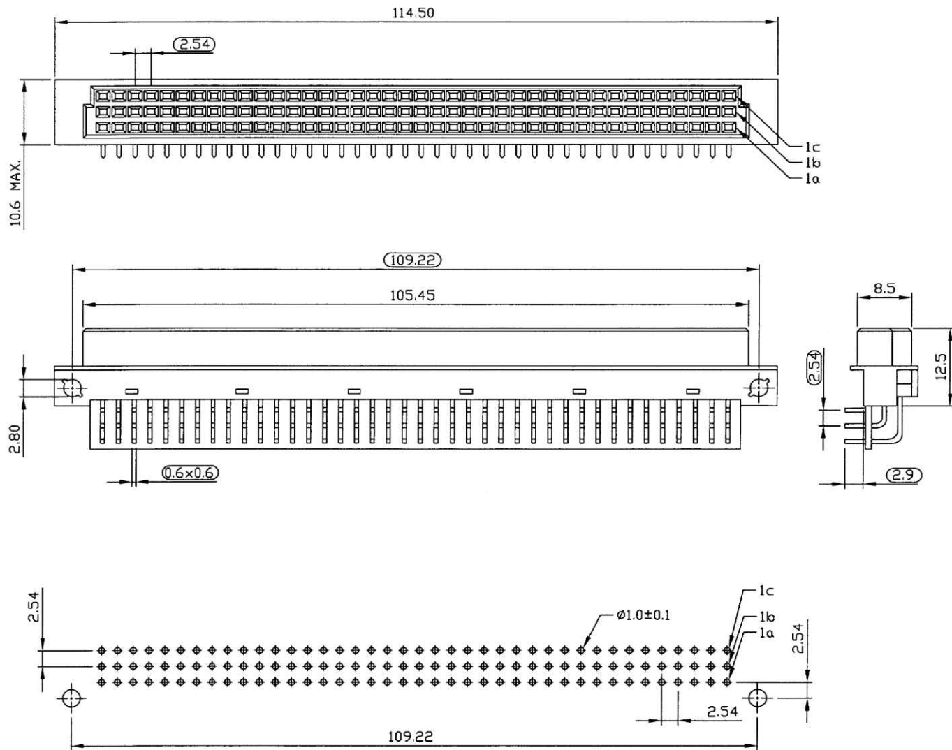
RECOMMENDED P.C.B LAYOUT(TOP VIEW) TOLERANCES: \pm 0.05\text{mm}
