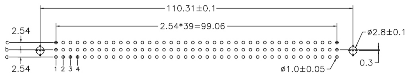
P.C. Board Layout
