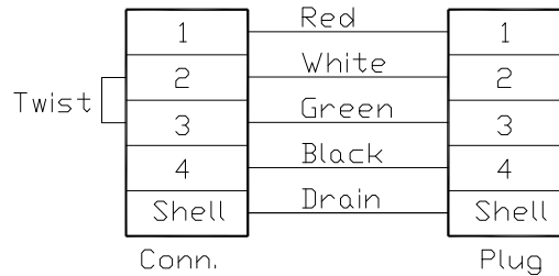
Wiring Diagram
