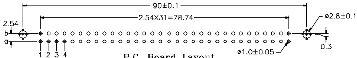
P.C. Board Layout
