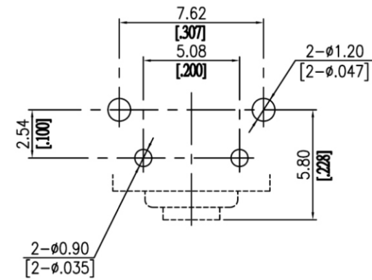
P.C.B. LAYOUT (VIEW FROM THE DIRECTION A)
