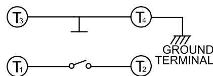
CIRCUIT DIAGRAM
