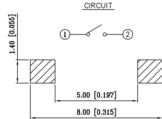
P.C.B. LAYOUT (VIEW FROM THE DIRECTION A)
