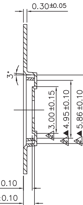
B-B Section
