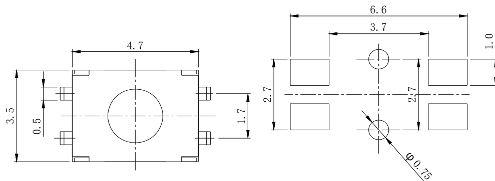
P. C. B PATTERN DIMENSION
