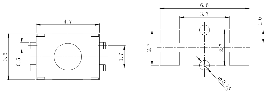
P. C. B PATTERN DIMENSION
