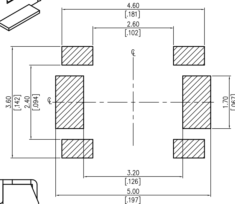
P.C.B. LAYOUT (VIEW FROM THE DIRECTION A)
