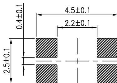
Recommended P.C.B Layout Solder thickness t=0.12^{+0.03}_{-0.02}
