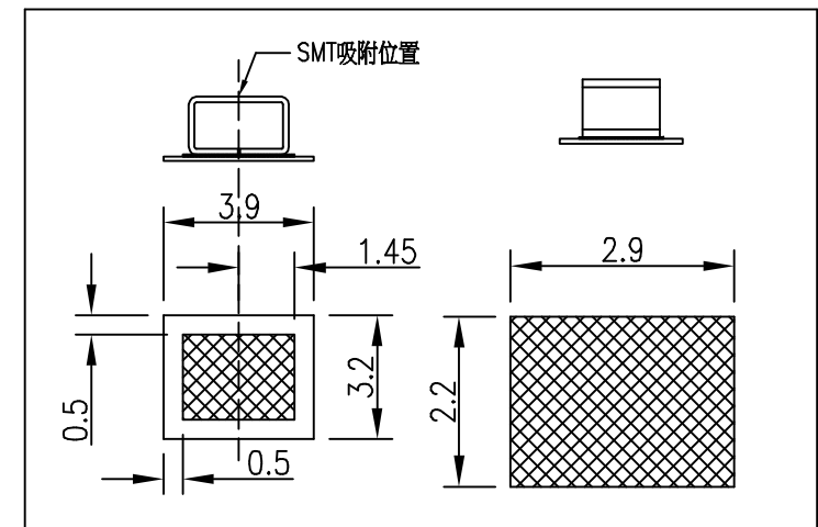
PCB Recommend Layout Pattern
