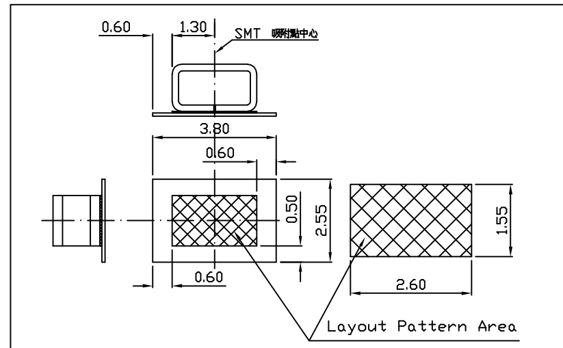
PCB Recommend Layout Pattern
