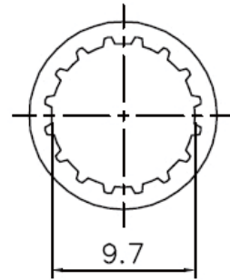
LOCK WASHER
