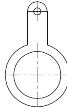
SOLDER TAG
