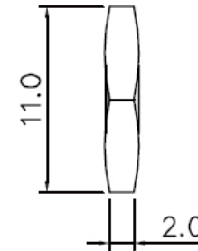
HEX. NUT
