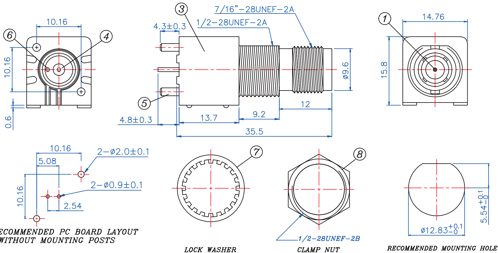
LOCK WASHER
