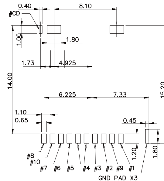
PCB LAYOUT
