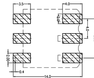
Board Layout
