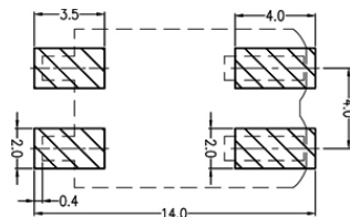
Board Layout
