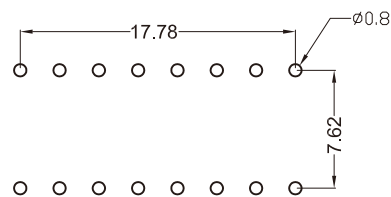
DRILLING PLAN
