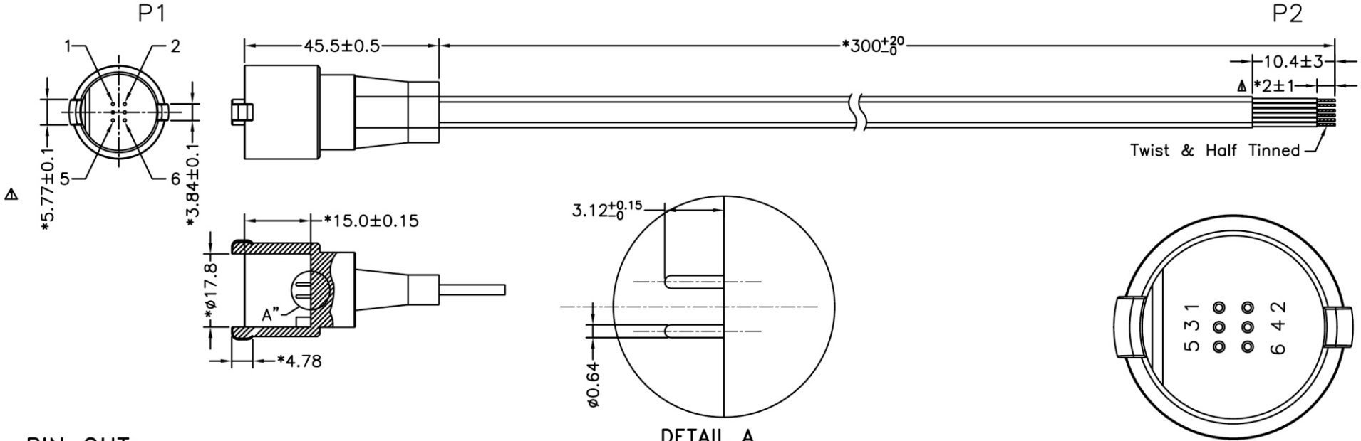
Front View
