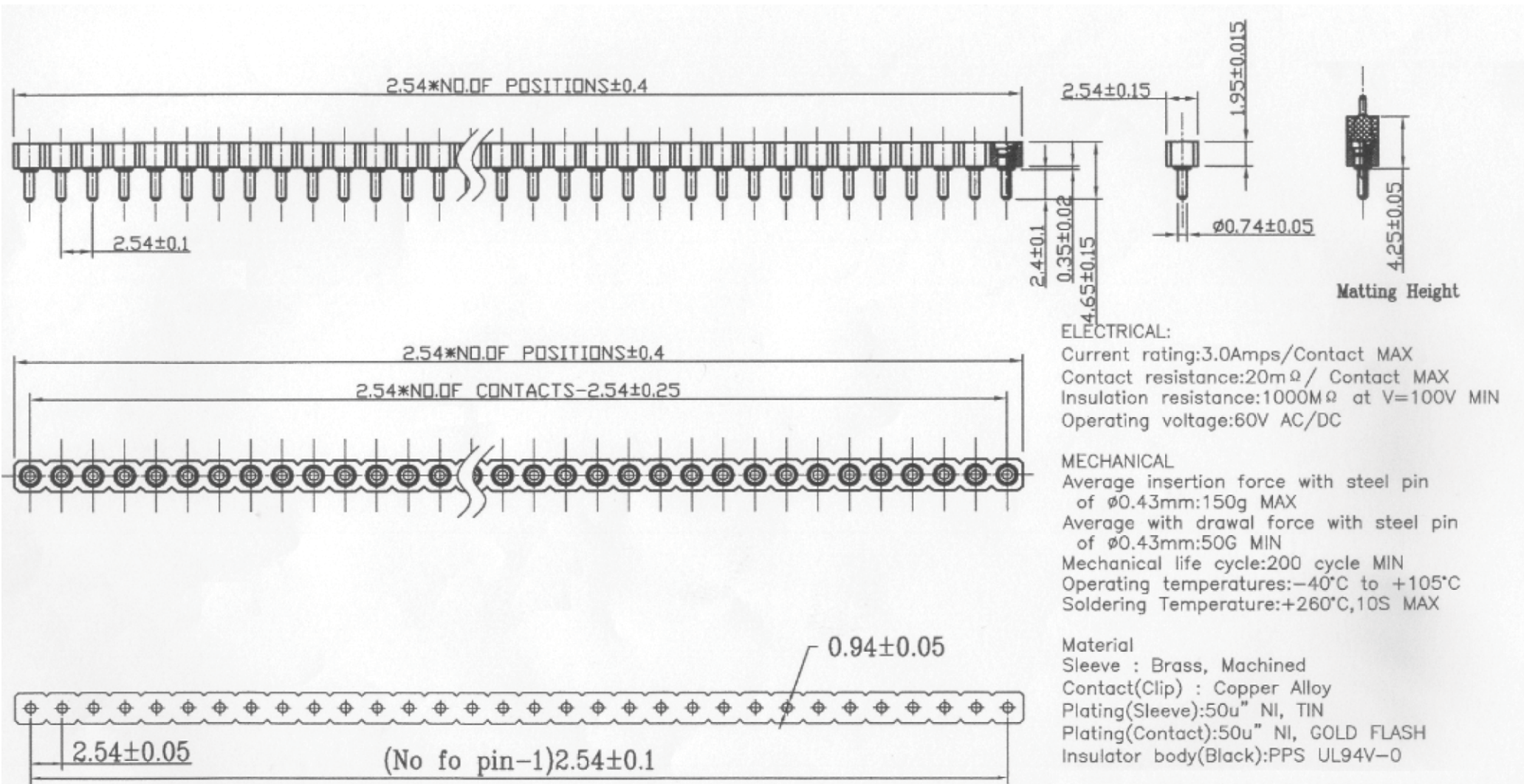
P. C. Board Layout
